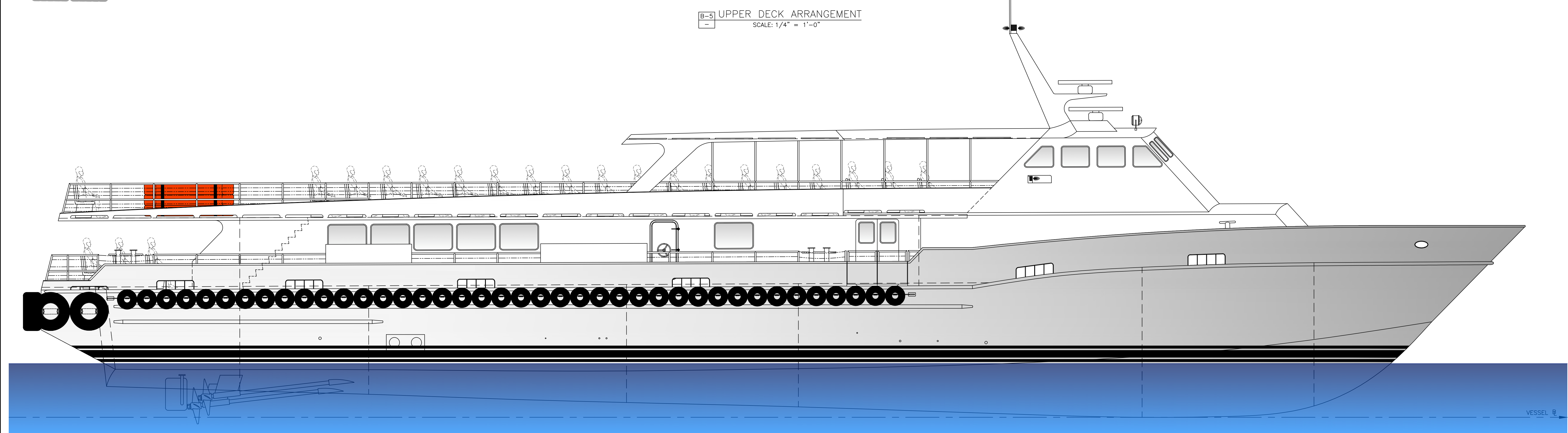
B-5 OUTBOARD PROFILE SCALE: 1/4" = 1'-0"
