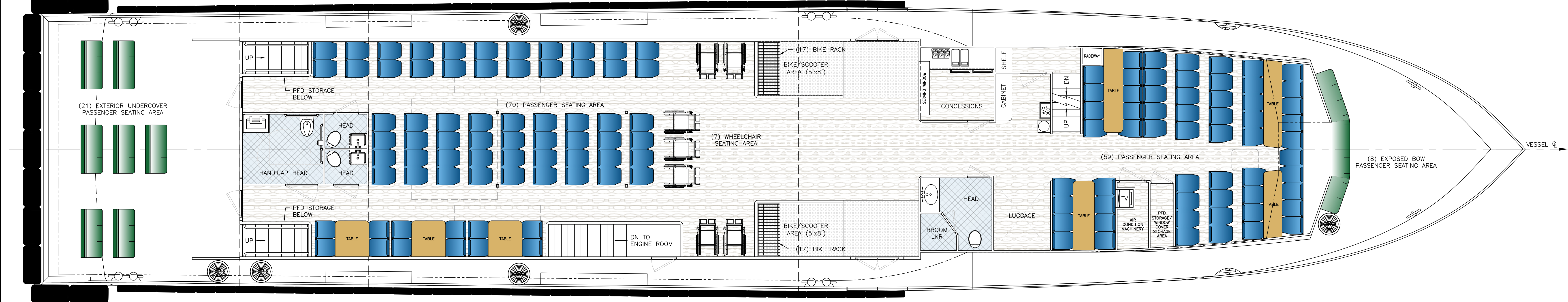
F-5 MAIN DECK ARRANGEMENT SCALE: 1/4" = 1'-0"
