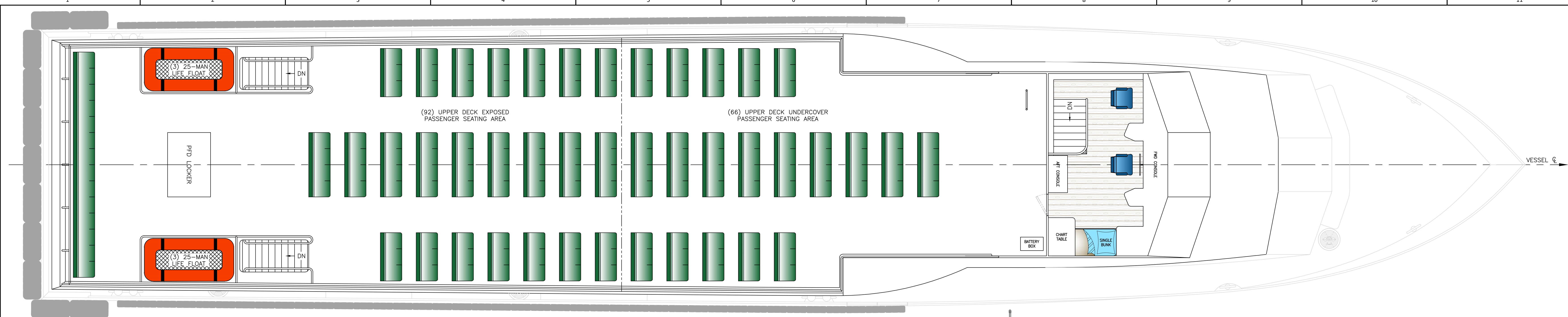
B-5 UPPER DECK ARRANGEMENT SCALE: 1/4" = 1'-0"
